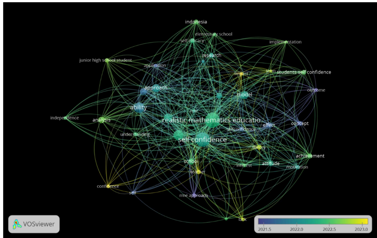
Figure 10. Visualization of Co-Occurrence Overlay Analysis on Research Related to RME, Self-Confidence, and Mathematics Education Curriculum Source: VOSviewer, 2024
