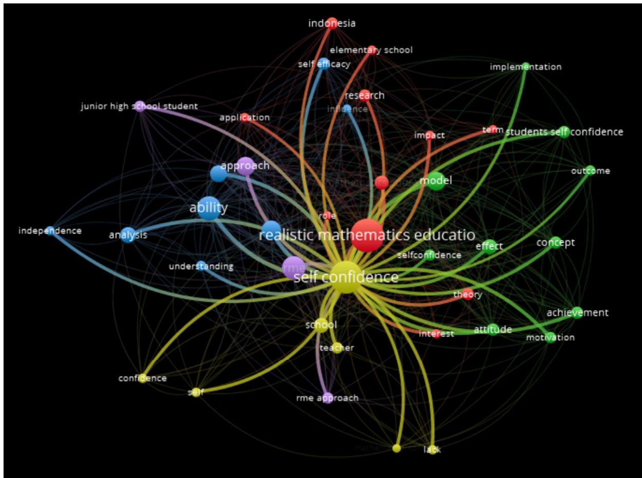
Figure 8. Visualization of Co-Occurrence Network Analysis in The Yellow Cluster Source: VOSviewer, 2024
