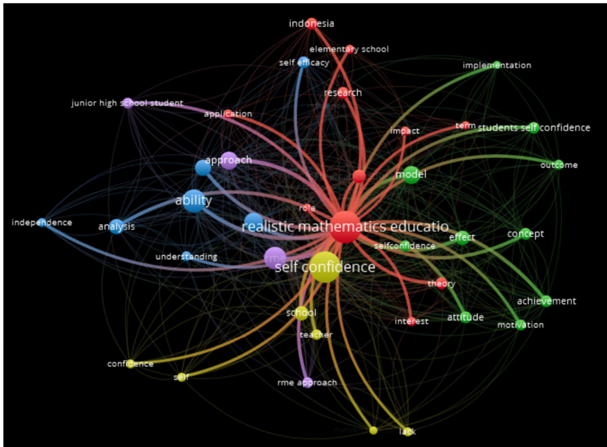
Figure 5. Visualization of Co-Occurrence Network Analysis in The Red Cluster Source: VOSviewer, 2024
